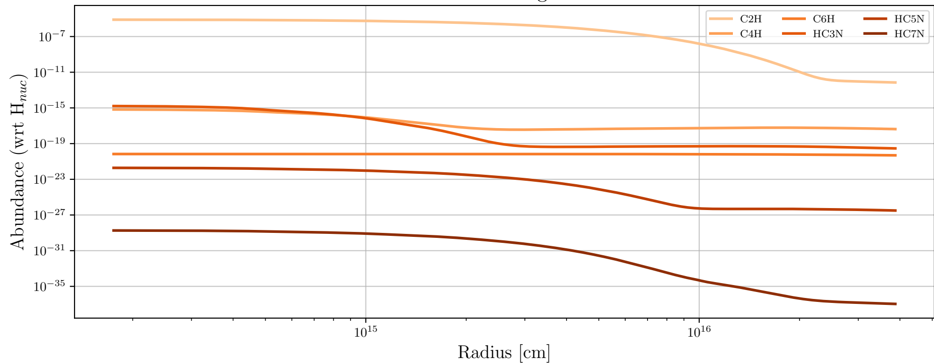
Particle 1188199 - Daughter Molecules
