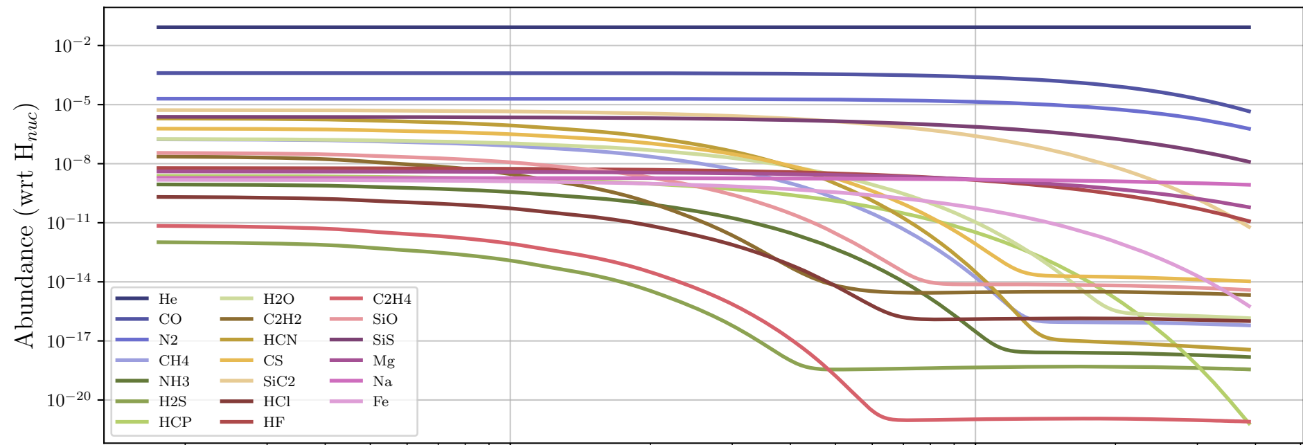
Particle 1188199 - Daughter Molecules
