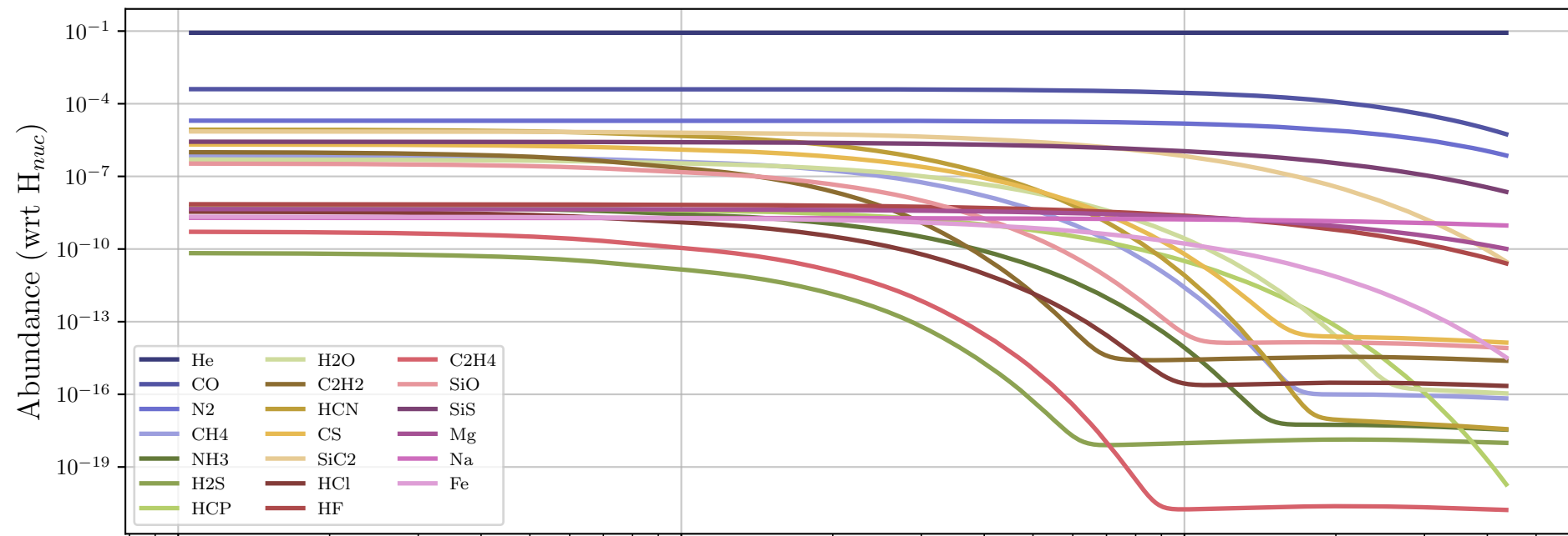
Particle 1477793 - Daughter Molecules
