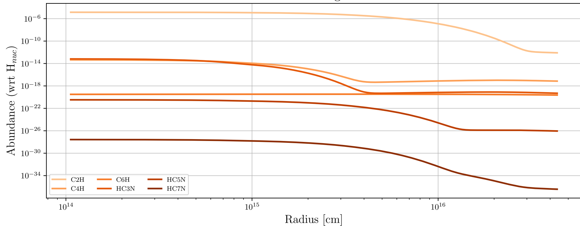
Particle 1477793 - Daughter Molecules
