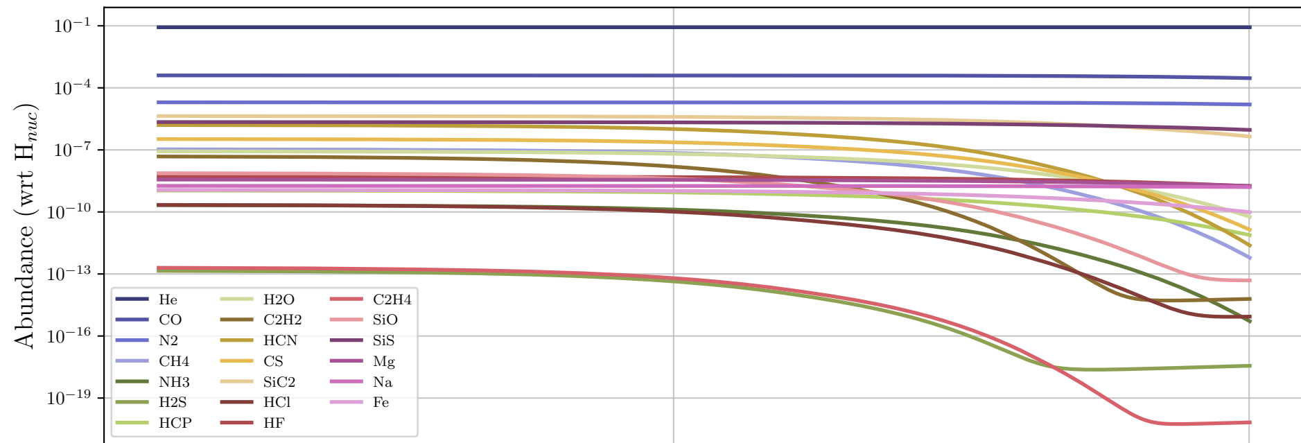
Particle 3538047 - Parent Molecules
