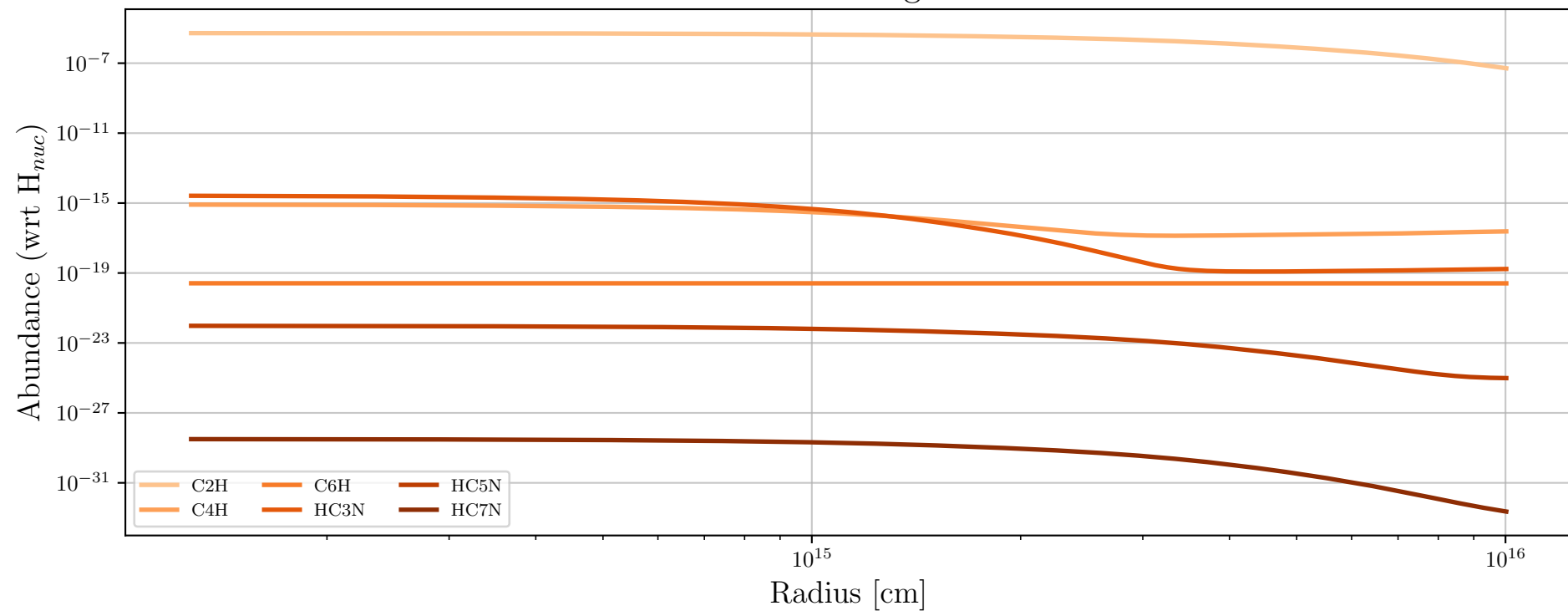
Particle 3538047 - Daughter Molecules
