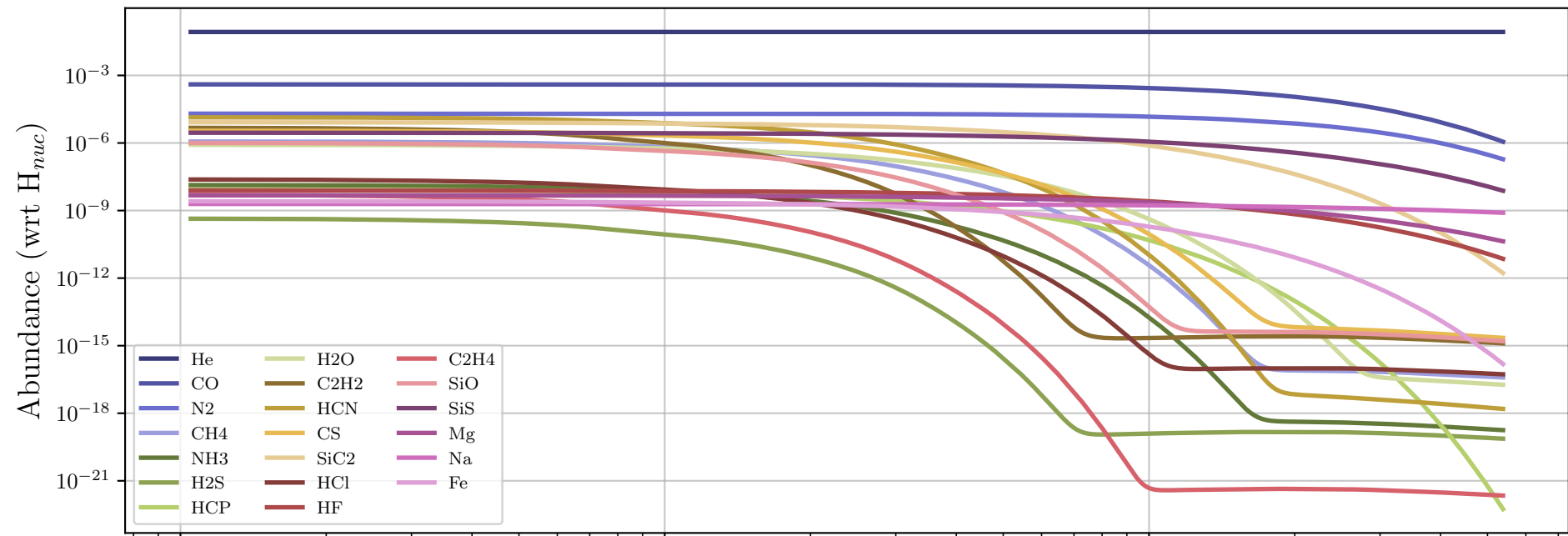
Particle 890331 - Daughter Molecules
