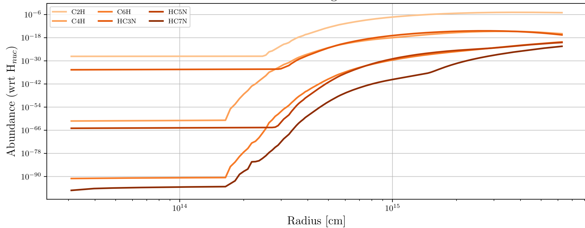
Particle 39353 - Daughter Molecules
