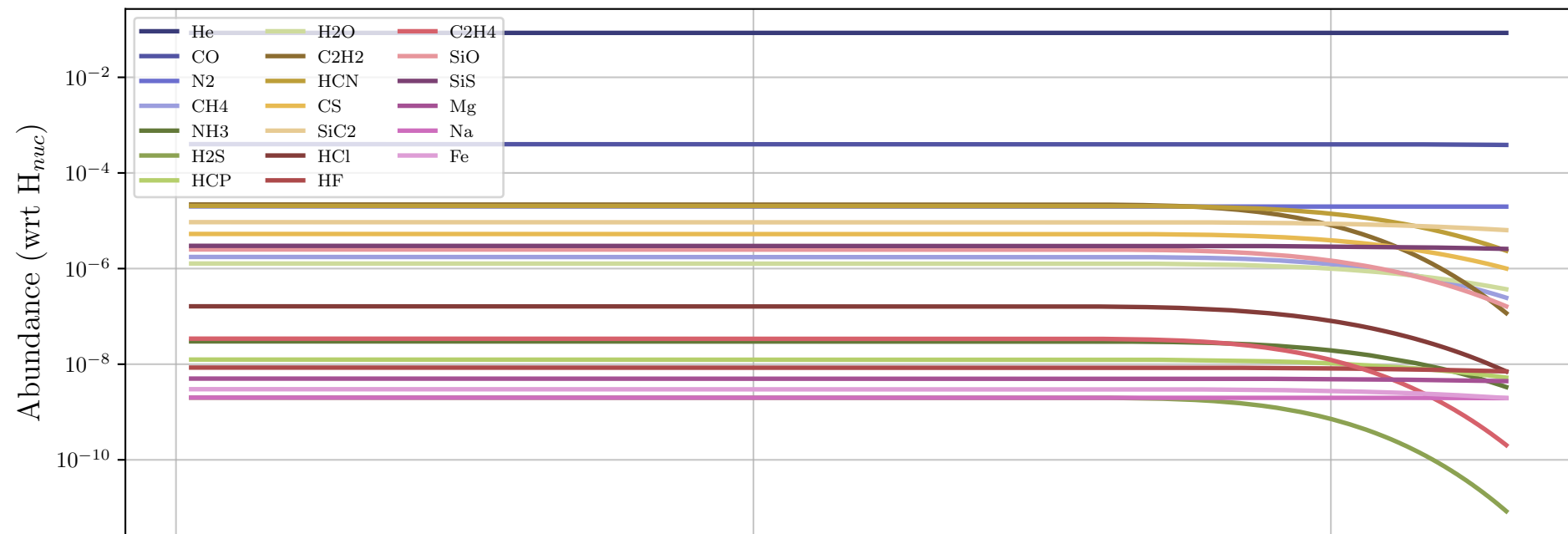
Particle 49168- Parent Molecules
