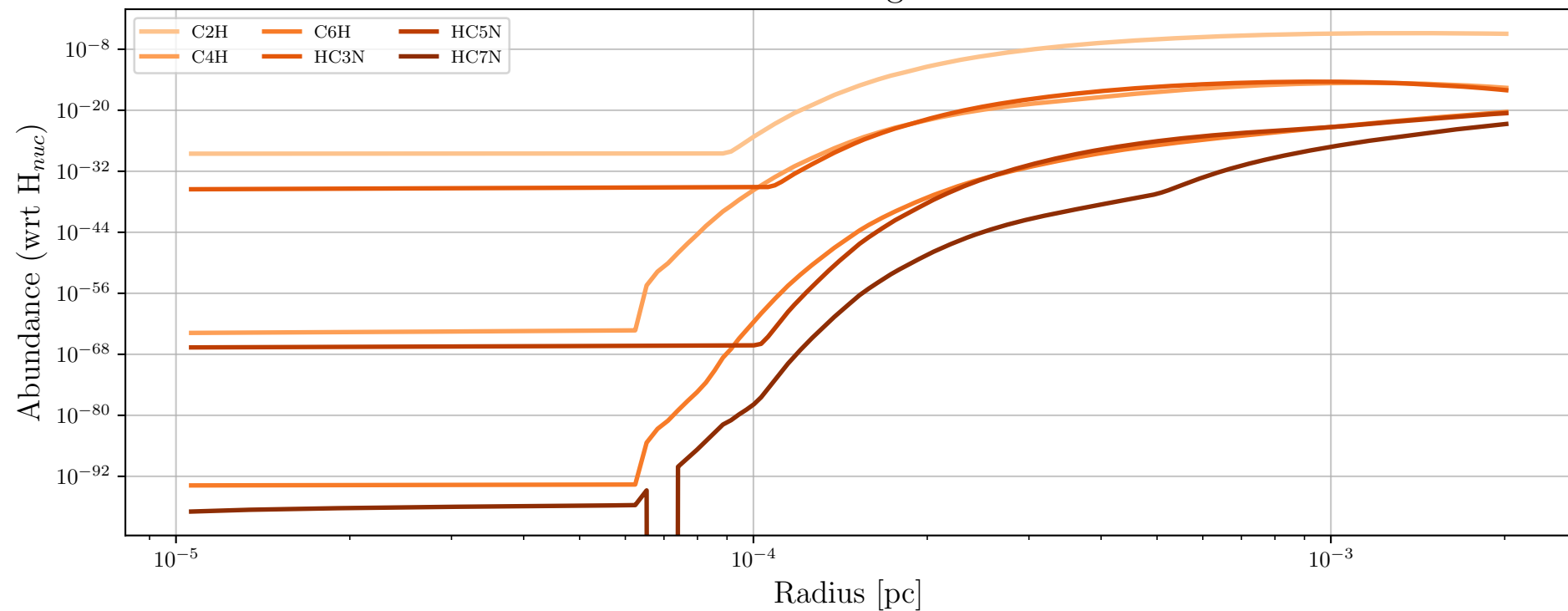
Particle 49168 - Daughter Molecules
