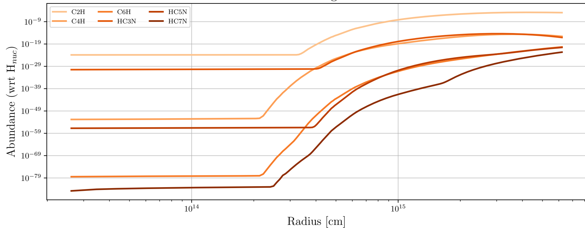
Particle 58983 - Daughter Molecules
