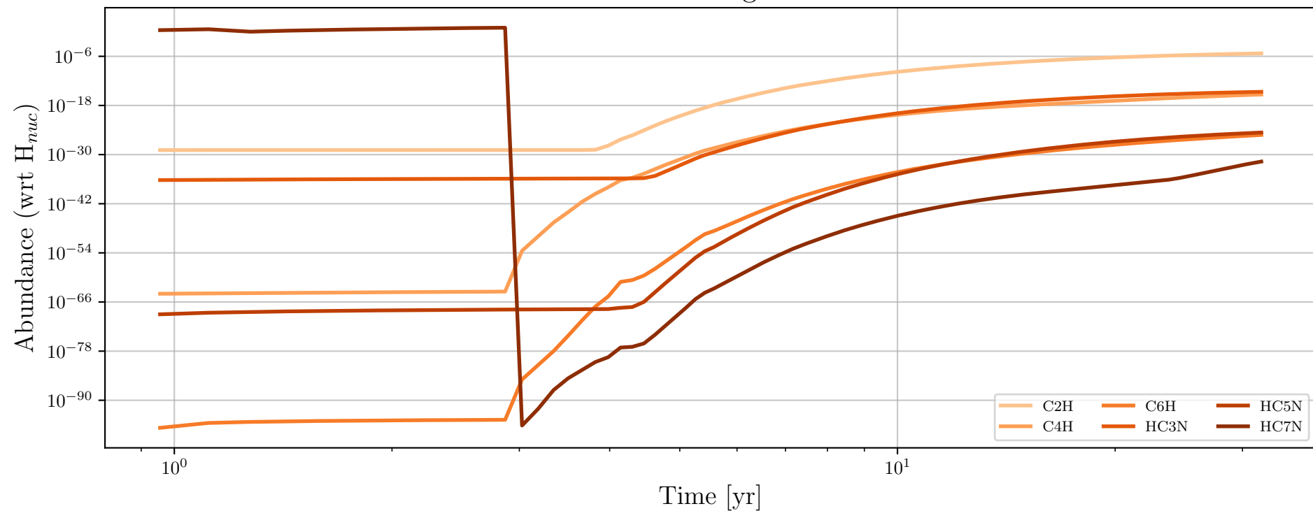
Particle 21810 - Daughter Molecules
