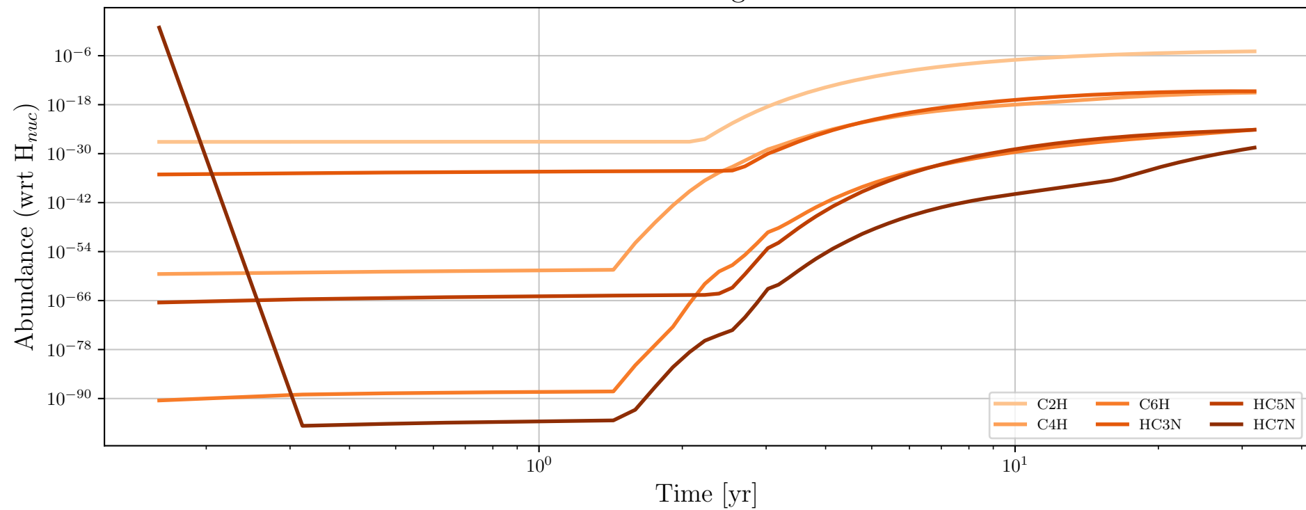
Particle 6401 - Daughter Molecules
