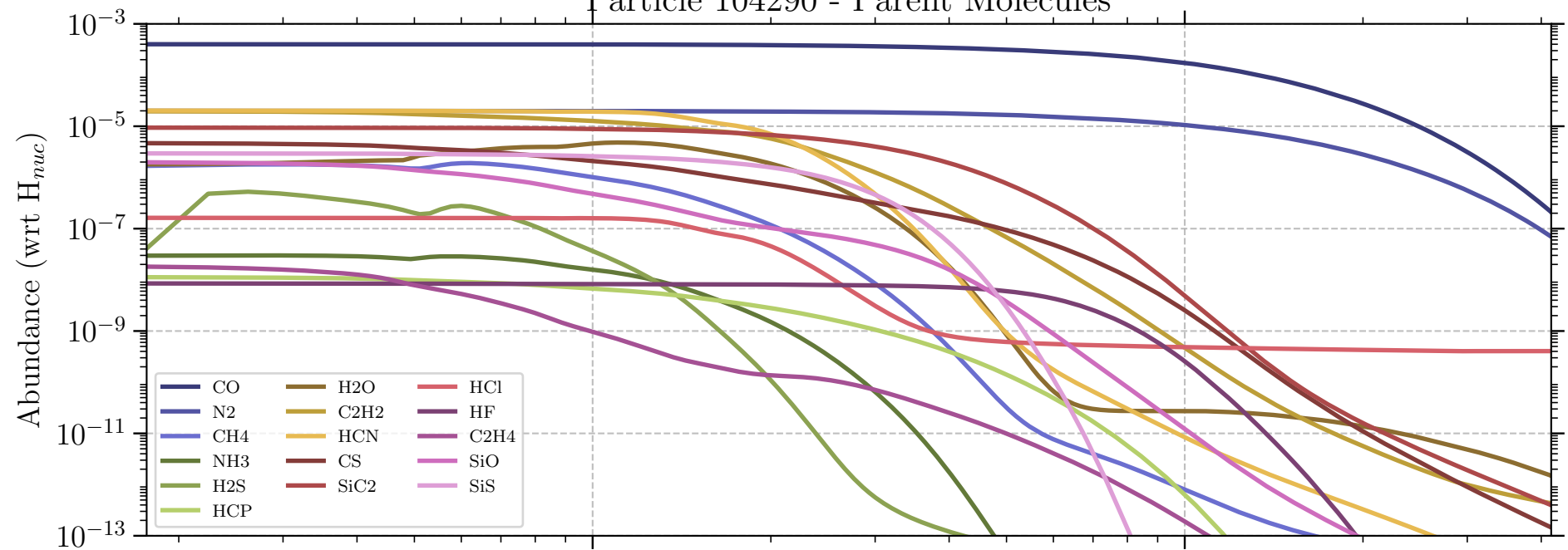
Particle 104290 - Daughter Molecules
