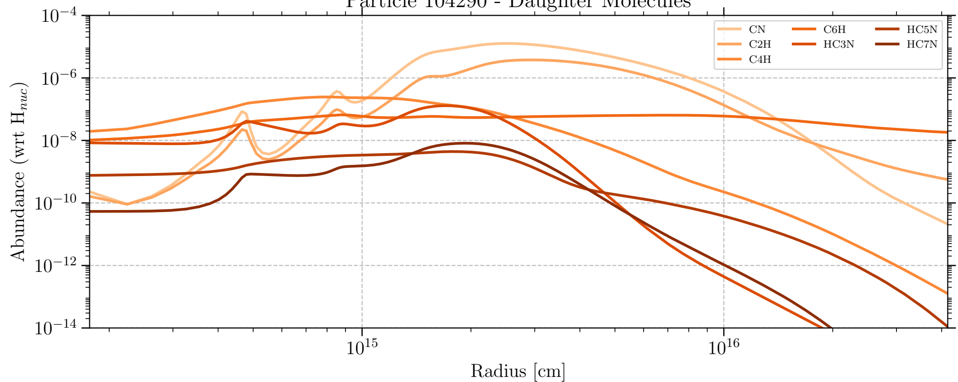
Particle 104290 - Daughter Molecules
