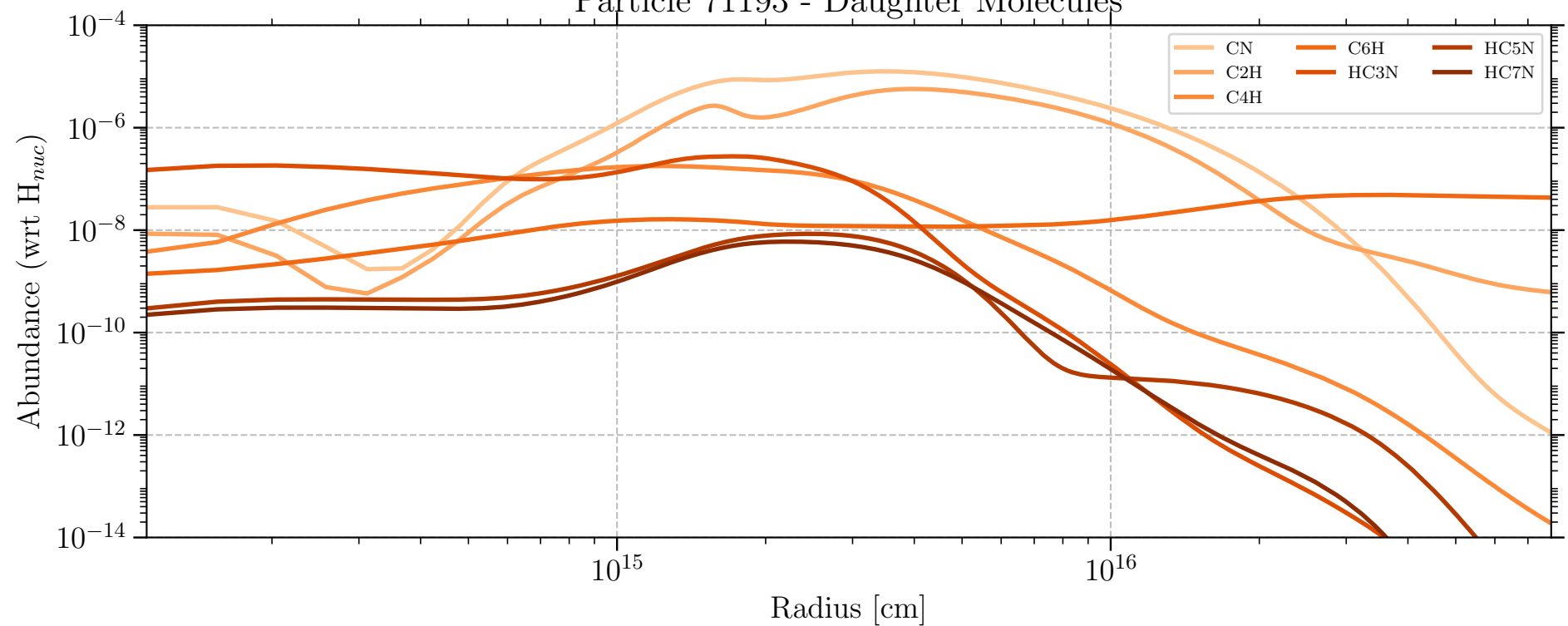
Particle 71193 - Daughter Molecules
