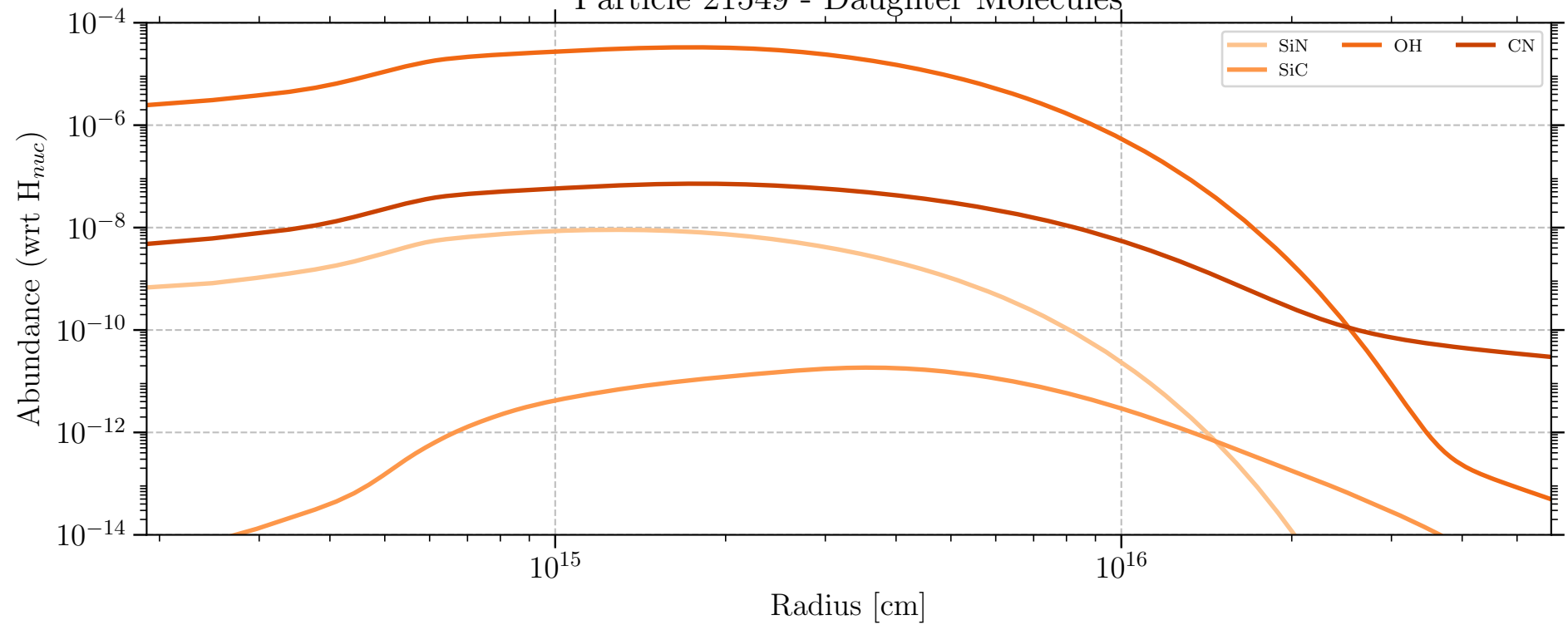
Particle 21549 - Daughter Molecules
