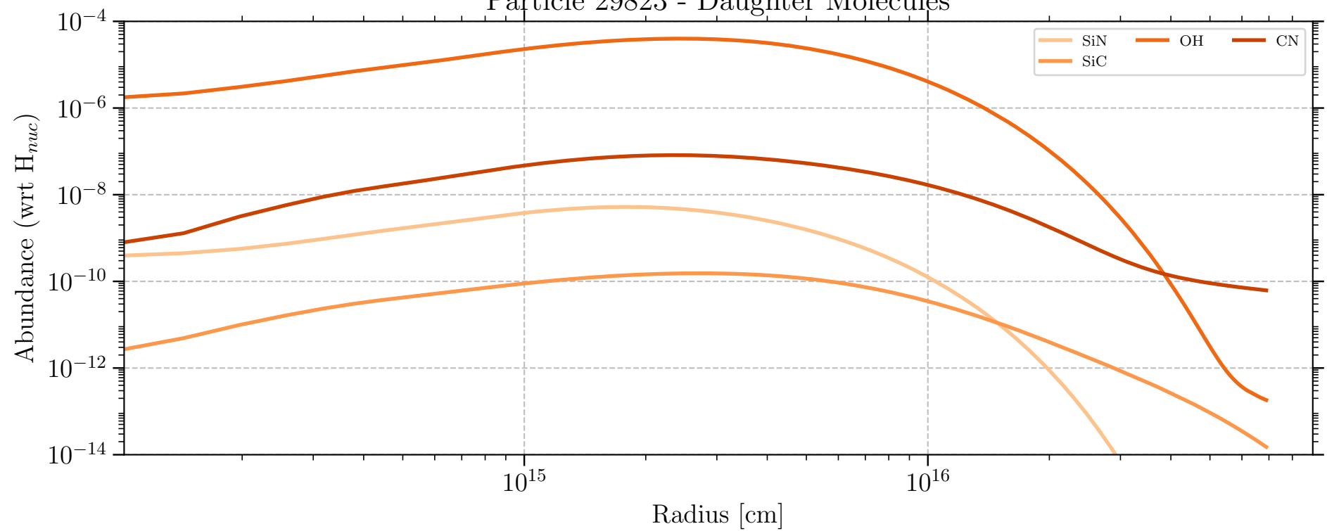
Particle 29823 - Daughter Molecules
