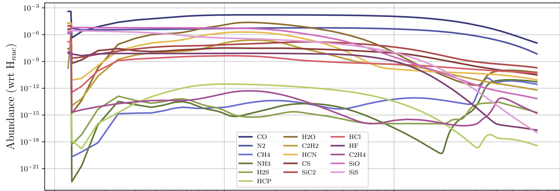
Particle 253224 - Daughter Molecules
