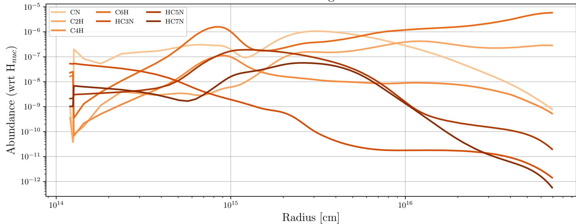
Particle 253224 - Daughter Molecules
