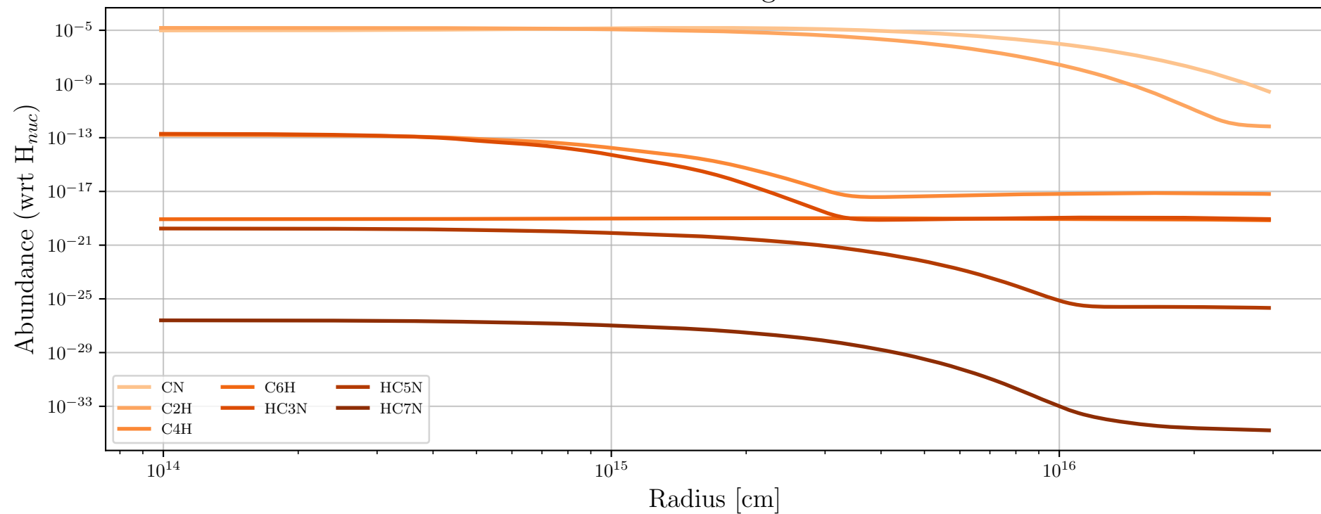
Particle 1775661 - Daughter Molecules
