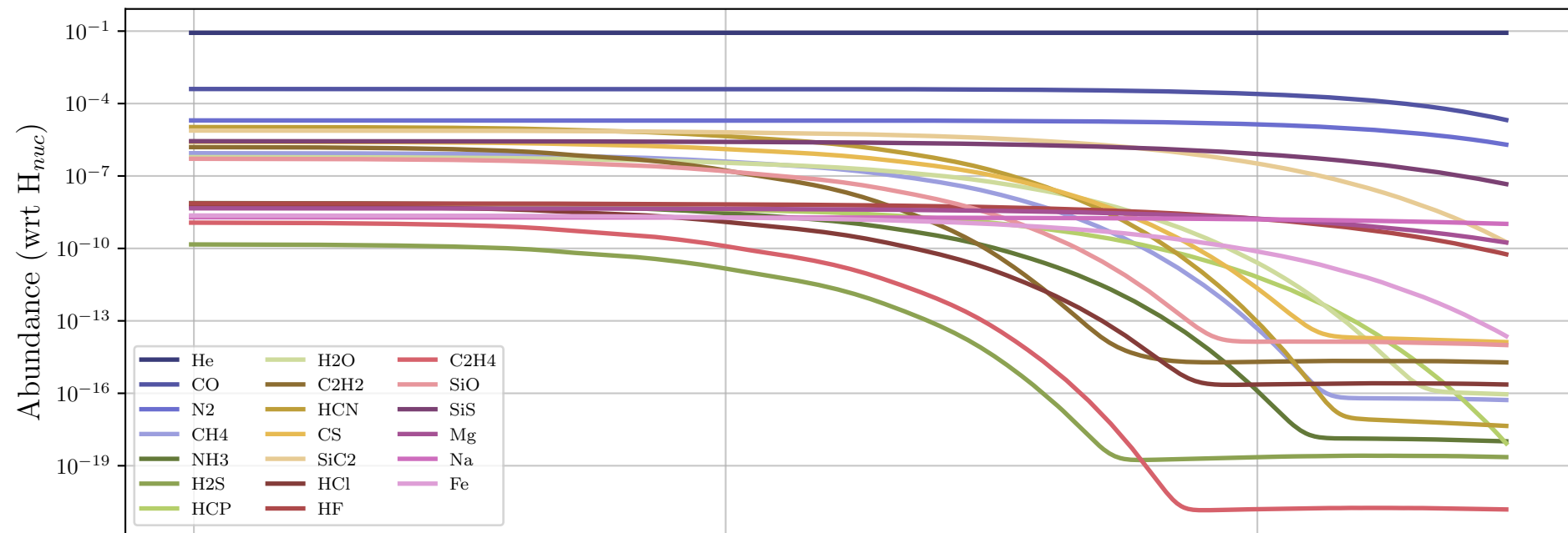
Particle 1775661 - Parent Molecules
