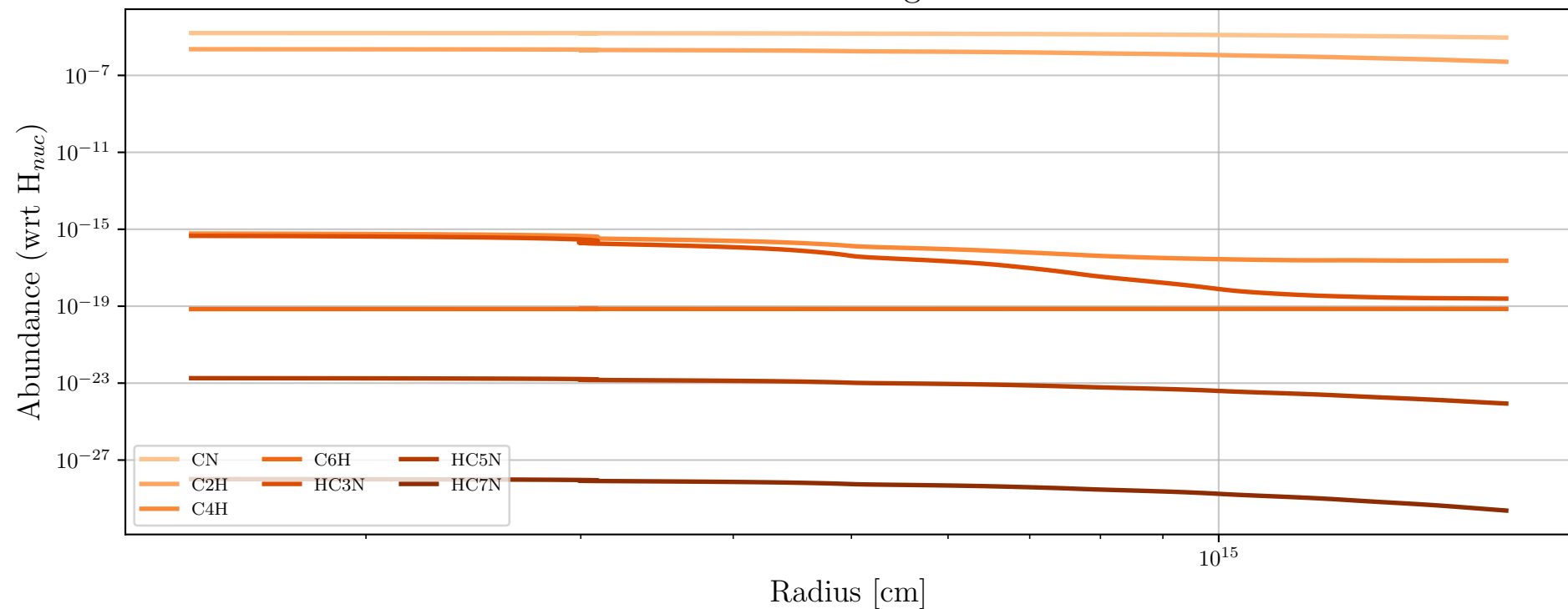
Particle 3827641 - Daughter Molecules
