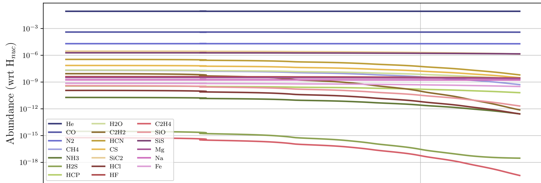
Particle 3827641 - Parent Molecules
