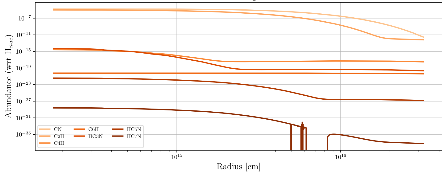
Particle 898605 - Daughter Molecules
