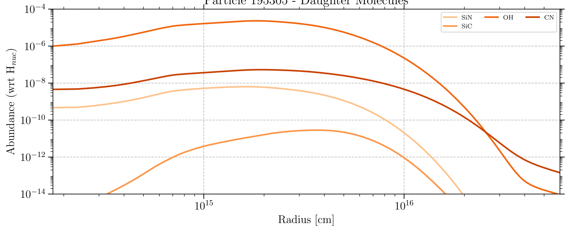
Particle 195305 - Daughter Molecules
