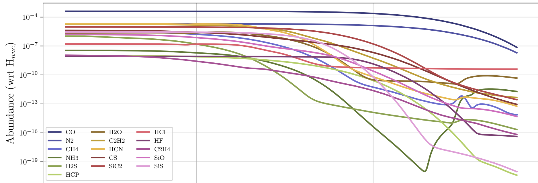
Particle 137386 - Parent Molecules
