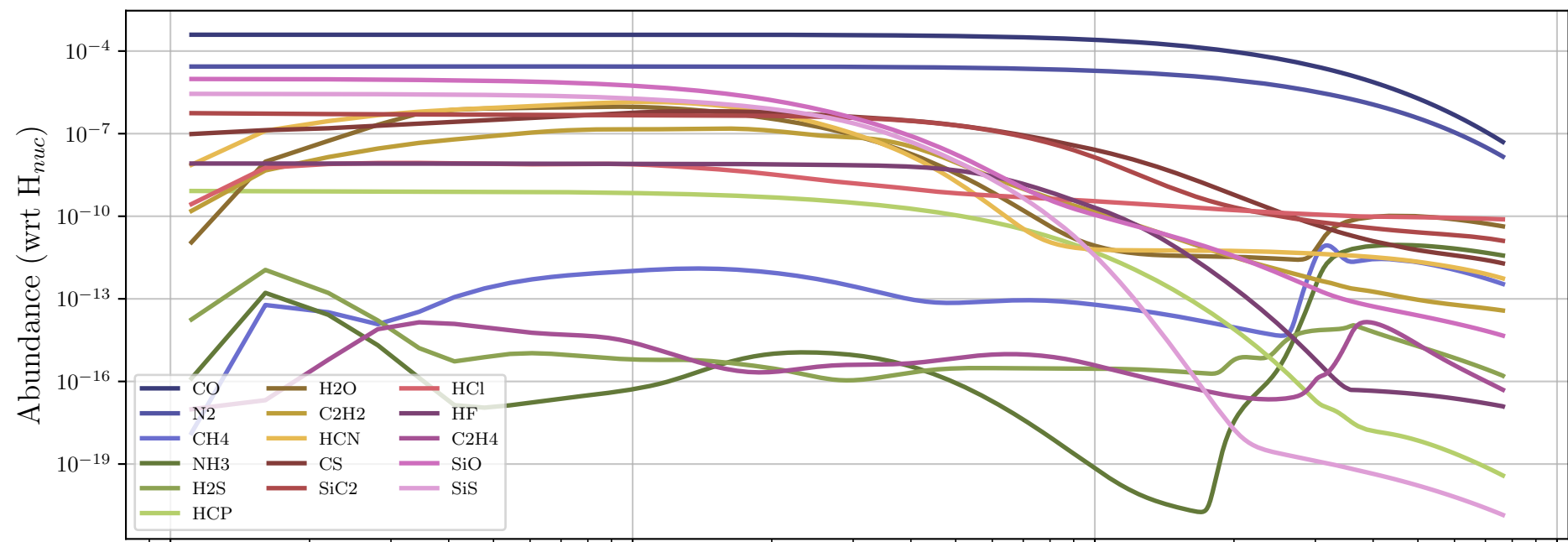
Particle 178757 - Daughter Molecules
