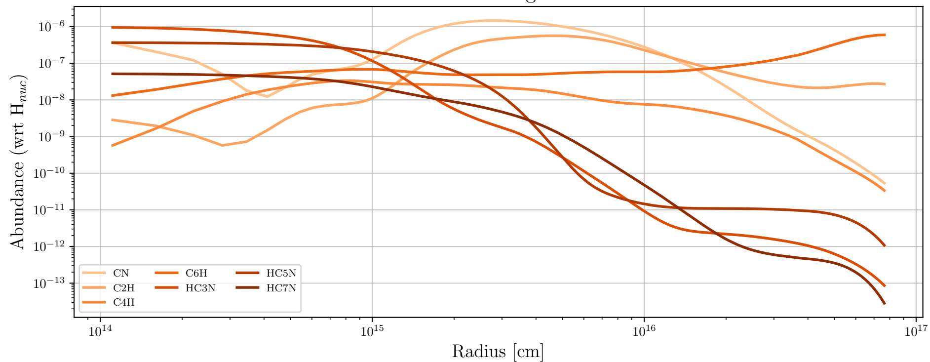
Particle 178757 - Daughter Molecules
