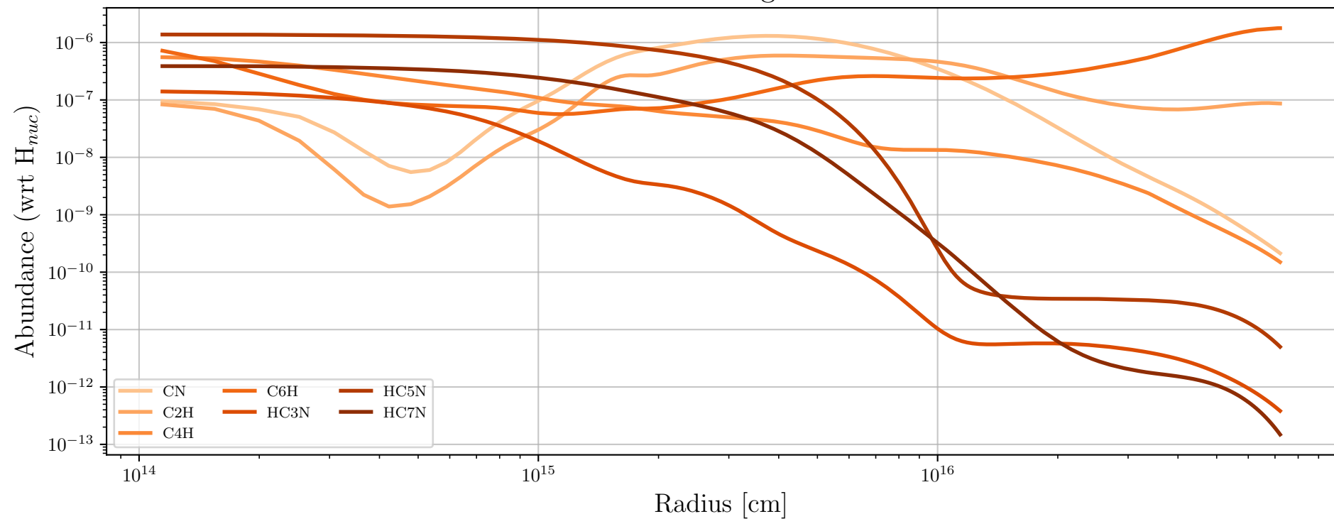
Particle 211853 - Daughter Molecules
