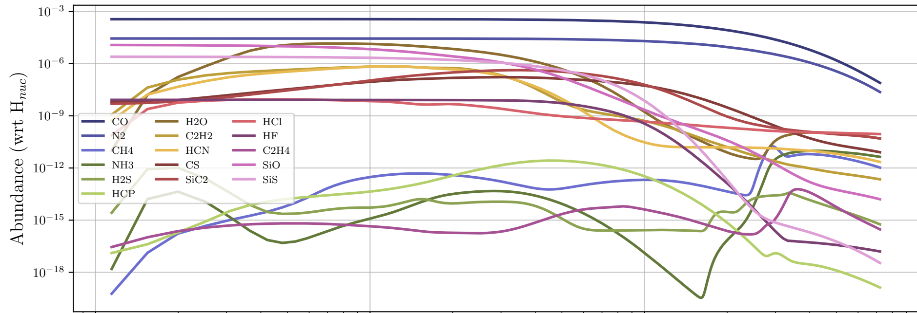
Particle 211853 - Daughter Molecules
