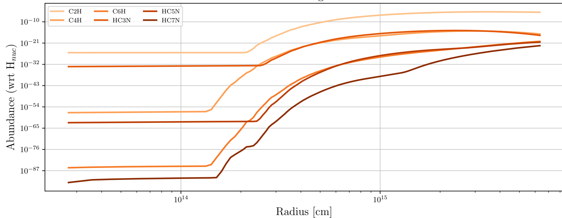
Particle 19723 - Daughter Molecules
