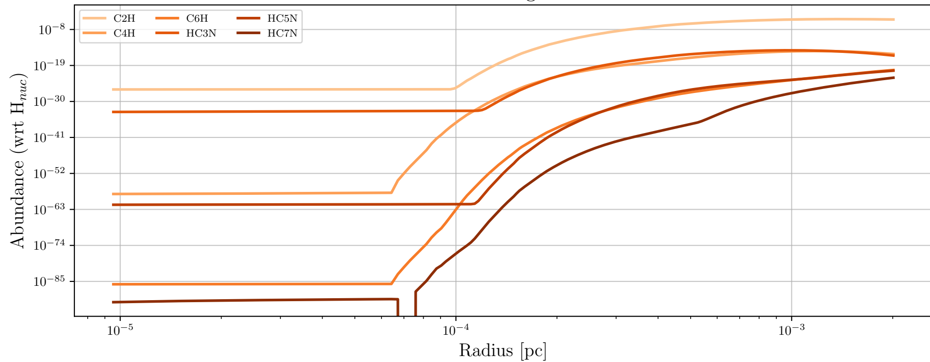
Particle 54076 - Daughter Molecules
