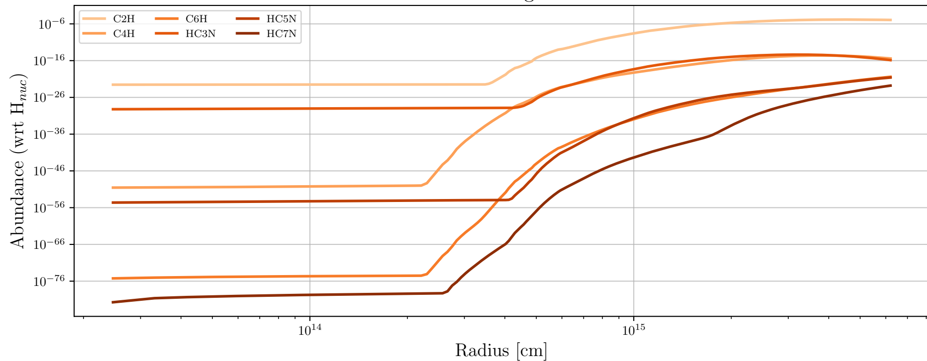
Particle 73706 - Daughter Molecules
