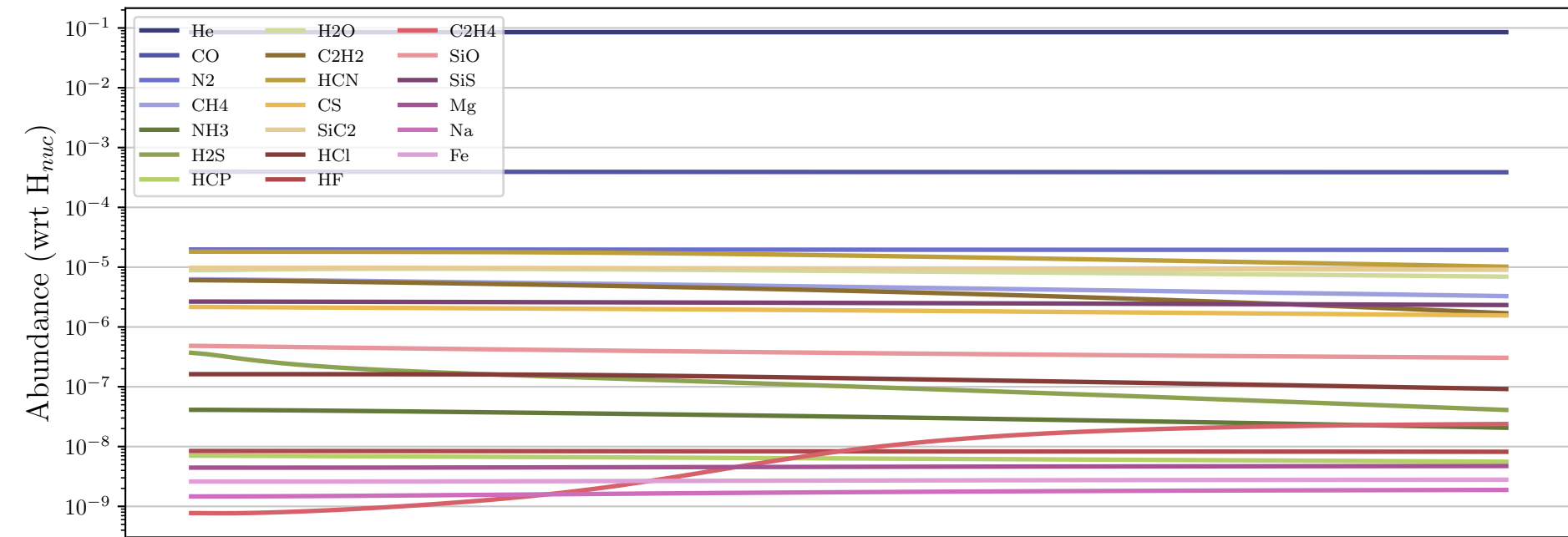
Particle 101515 - Daughter Molecules
