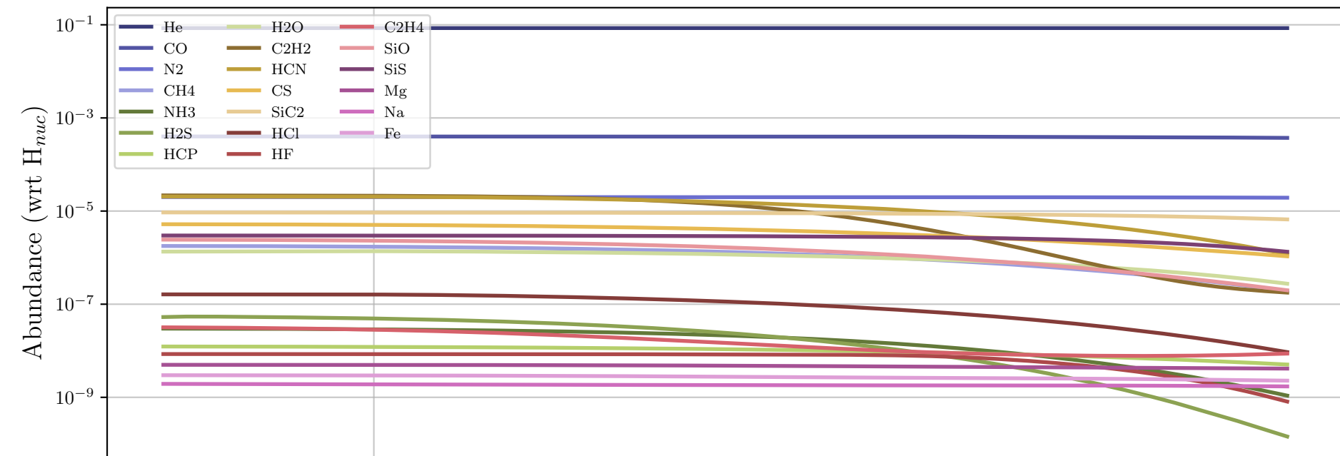
Particle 13775- Parent Molecules
