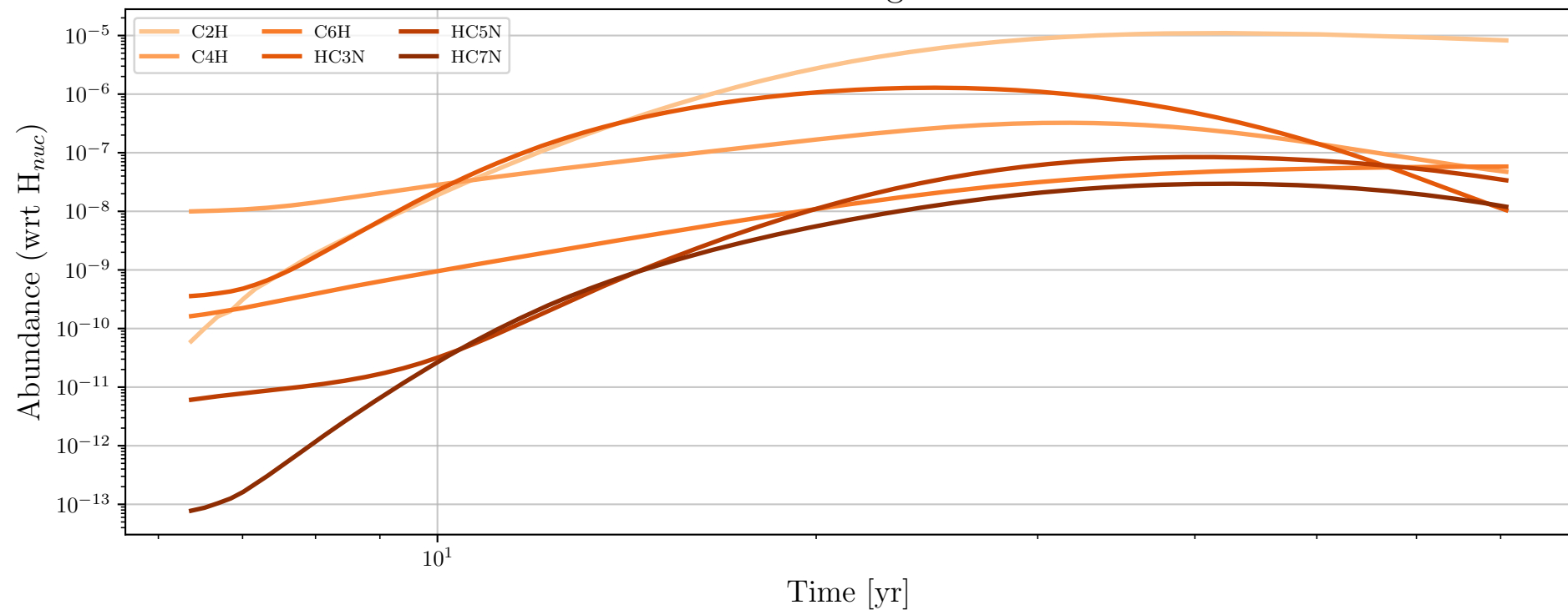
Particle 13775 - Daughter Molecules
