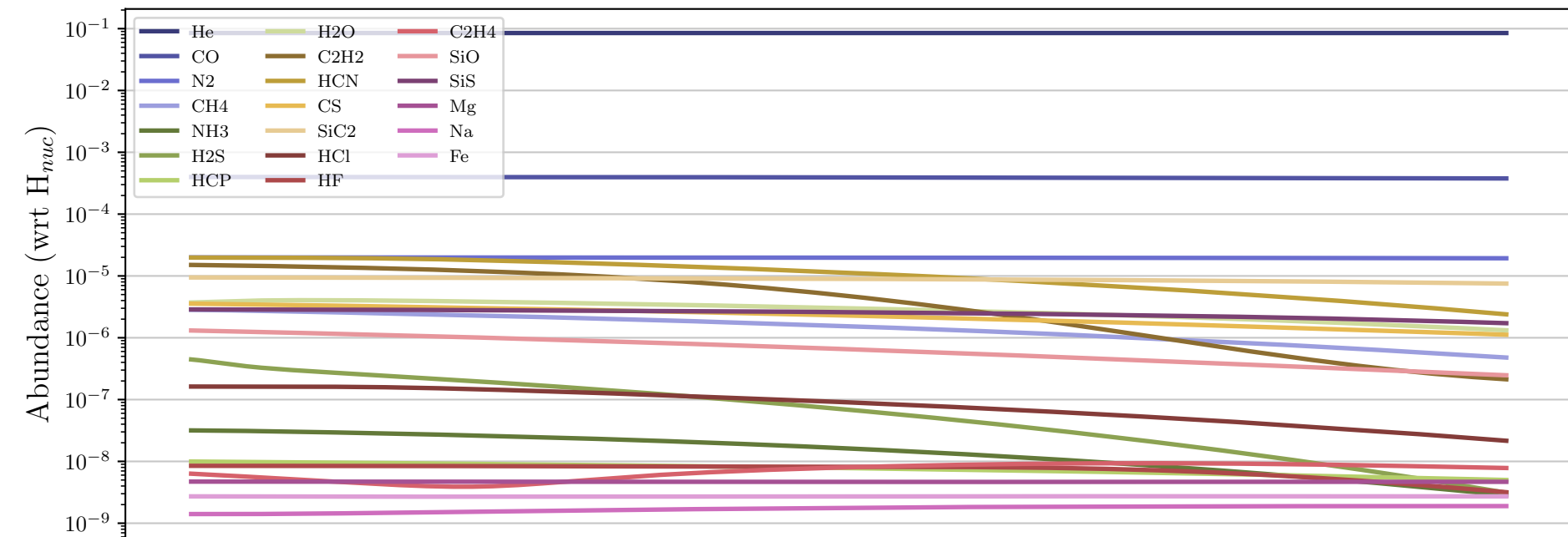
Particle 48871 - Daughter Molecules
