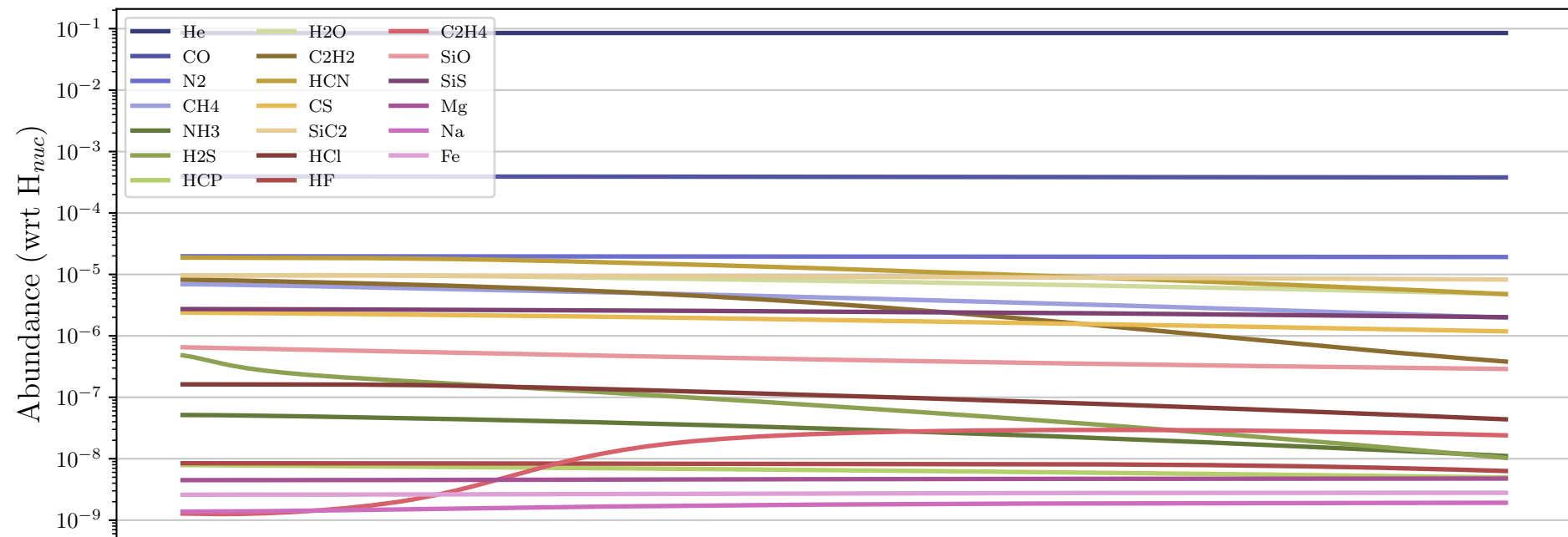
Particle 75193 - Daughter Molecules
