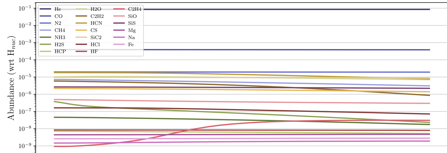
Particle 92741 - Daughter Molecules
