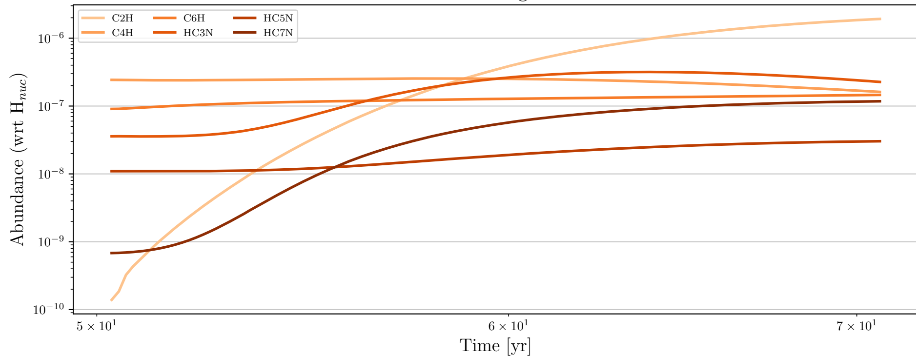
Particle 92741 - Daughter Molecules
