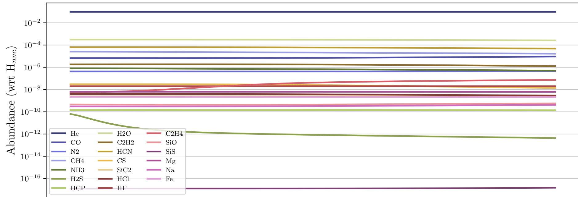
Particle 110289 - Daughter Molecules
