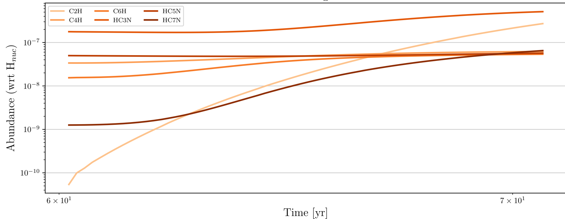
Particle 110289 - Daughter Molecules
