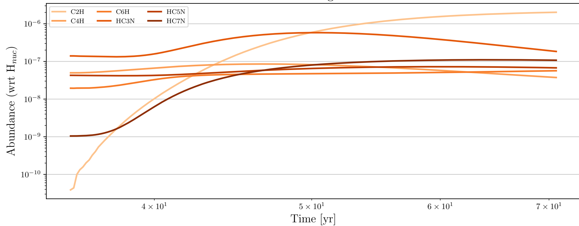
Particle 66419 - Daughter Molecules
