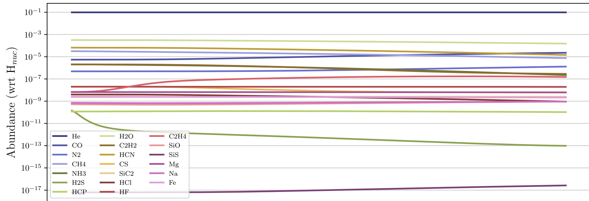
Particle 66419 - Daughter Molecules
