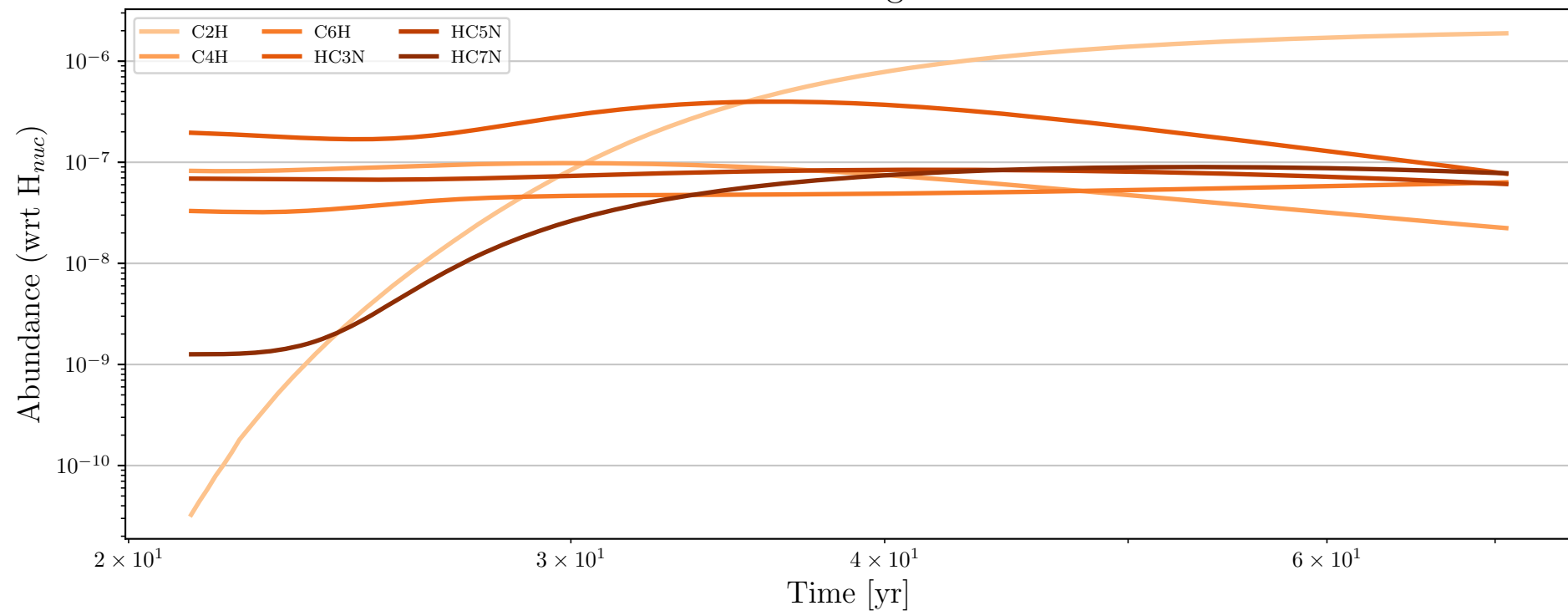
Particle 40097 - Daughter Molecules
