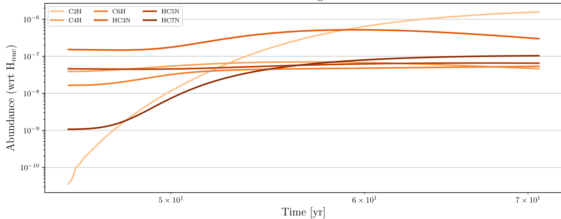
Particle 83967 - Daughter Molecules
