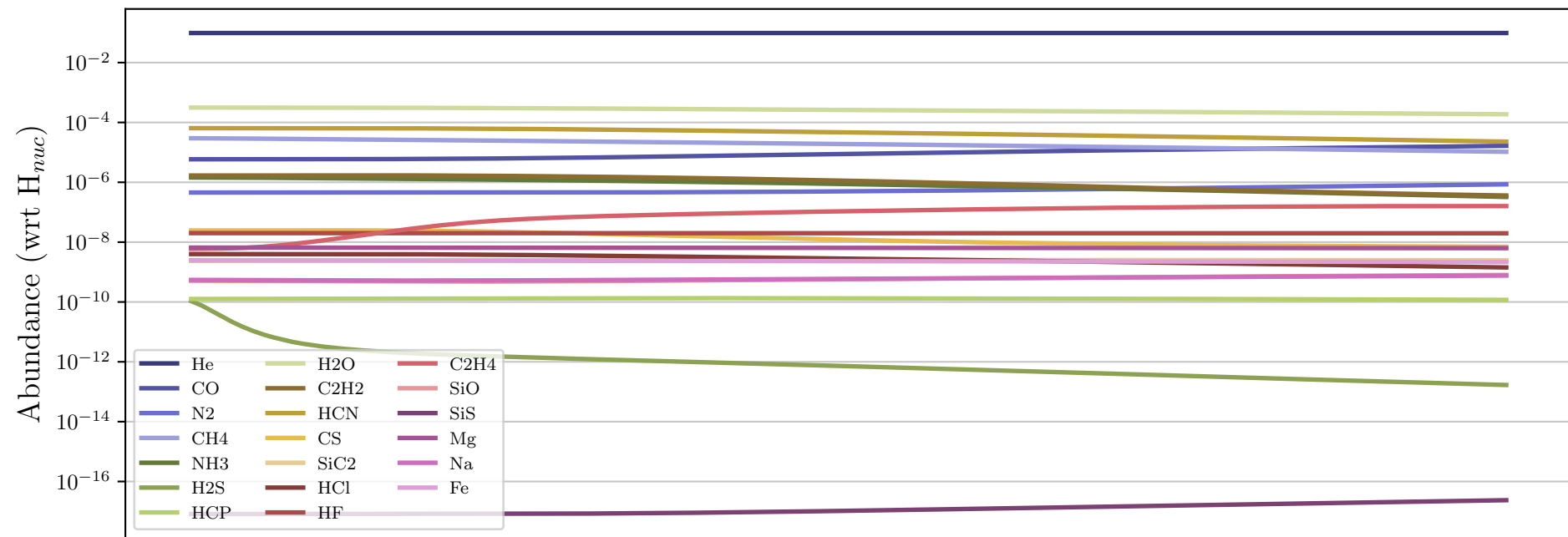
Particle 83967 - Daughter Molecules
