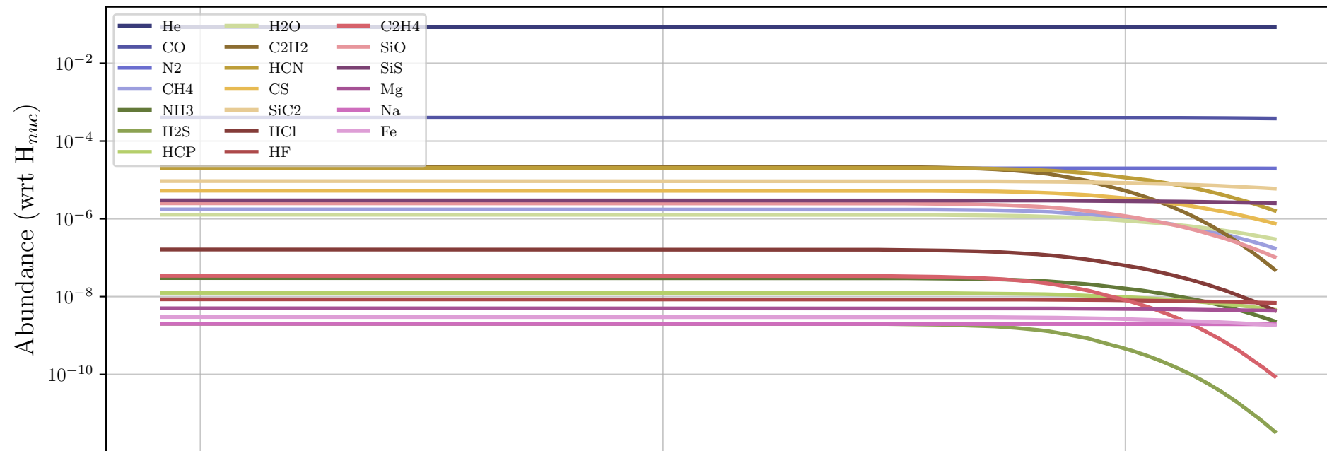
Particle 9908 - Parent Molecules
