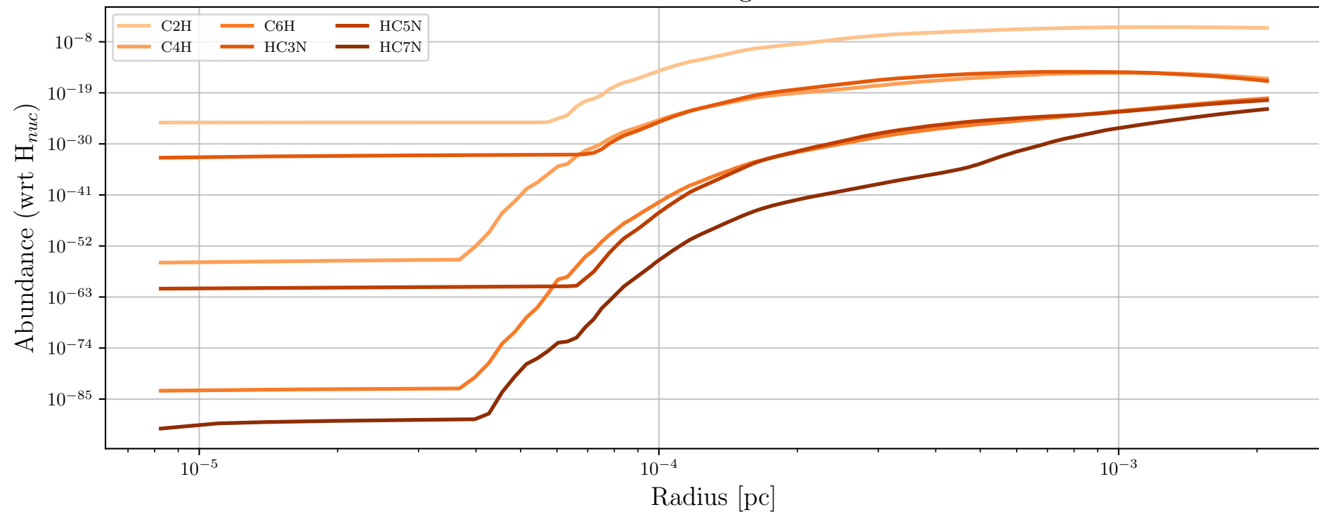
Particle 9908 - Daughter Molecules
