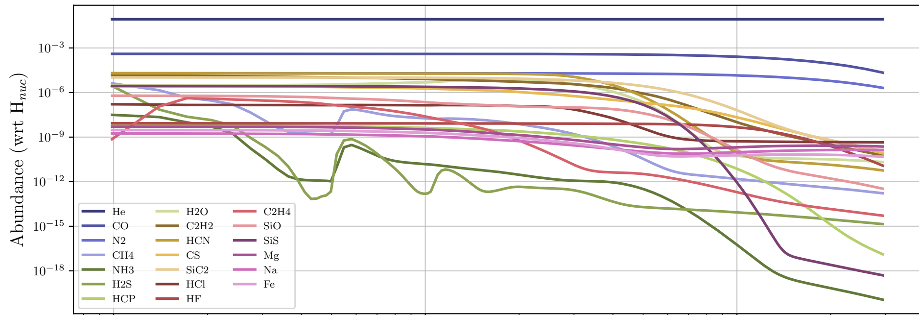
Particle 1775661 - Daughter Molecules
