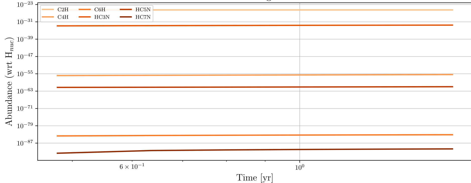
Particle 13631 - Daughter Molecules
