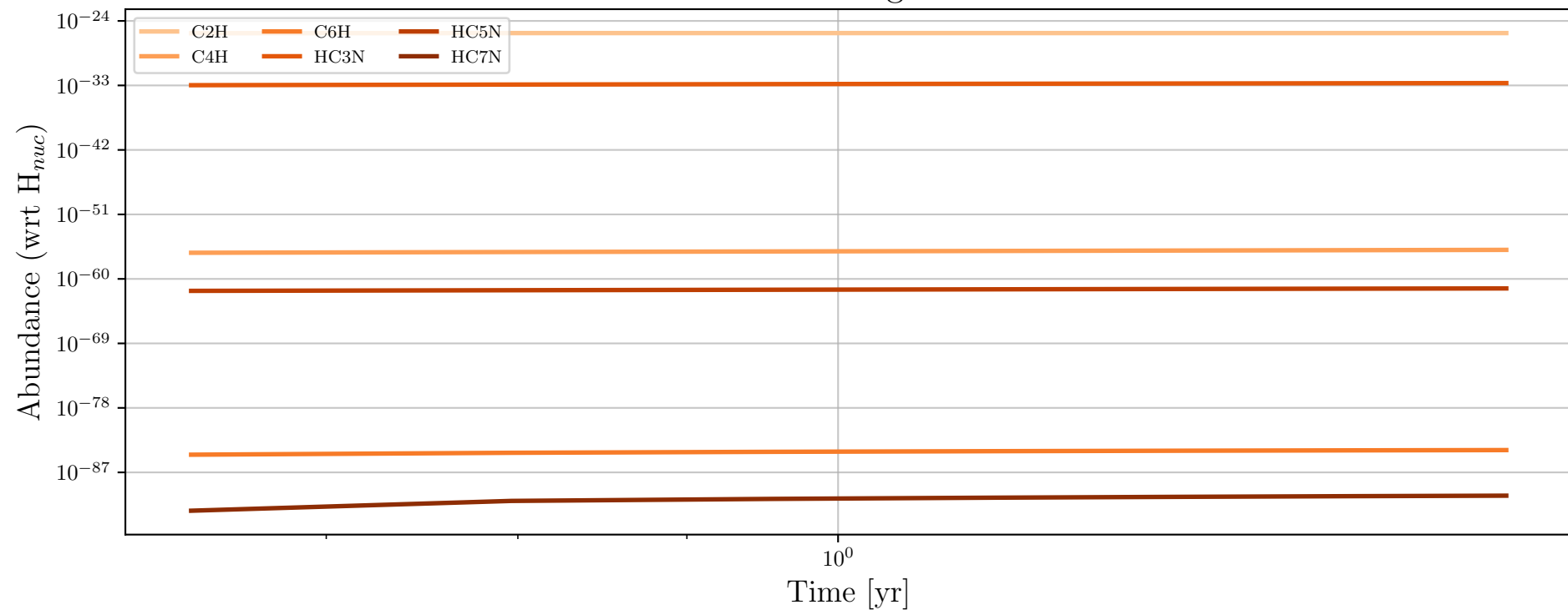
Particle 16357 - Daughter Molecules
