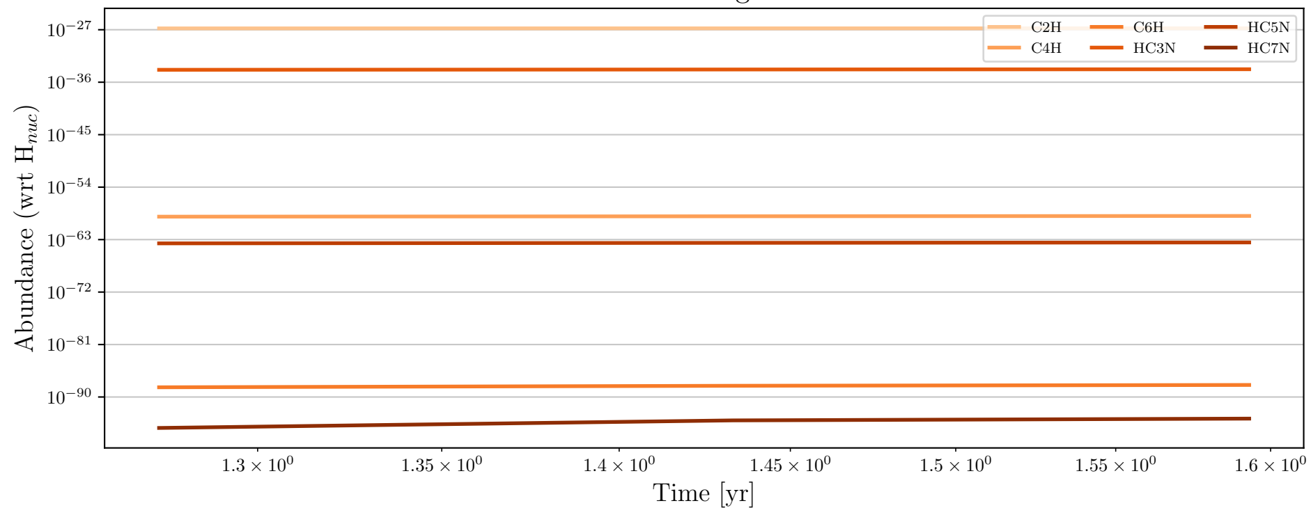
Particle 29986 - Daughter Molecules
