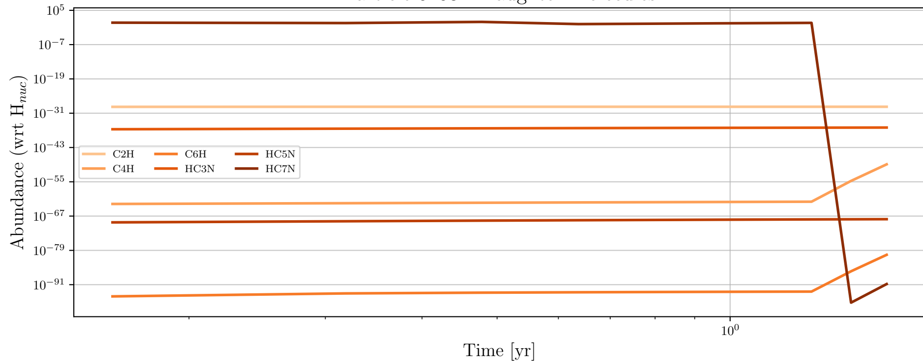
Particle 5453 - Daughter Molecules
