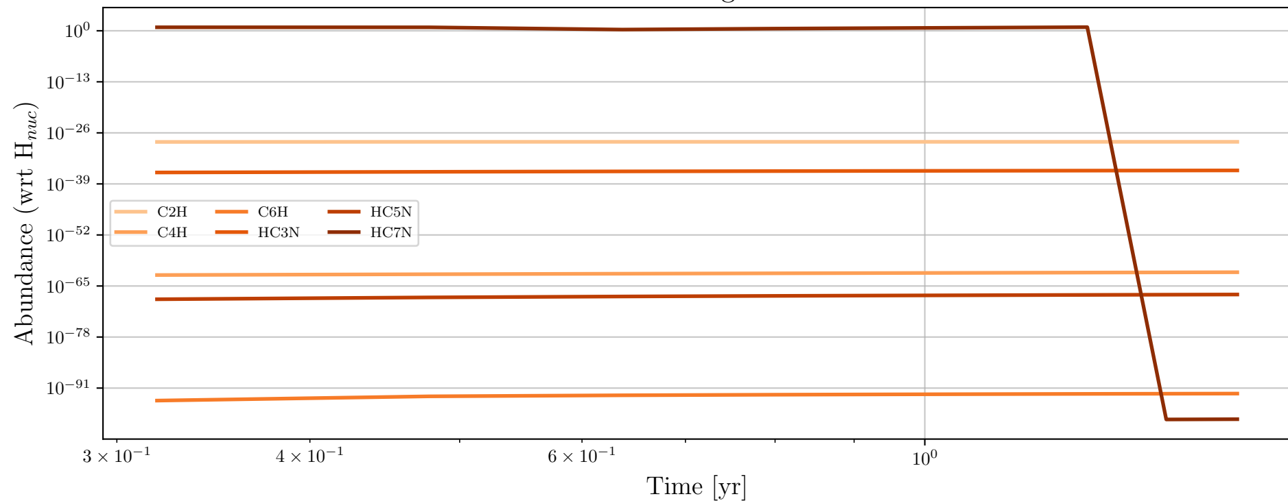
Particle 8179 - Daughter Molecules
