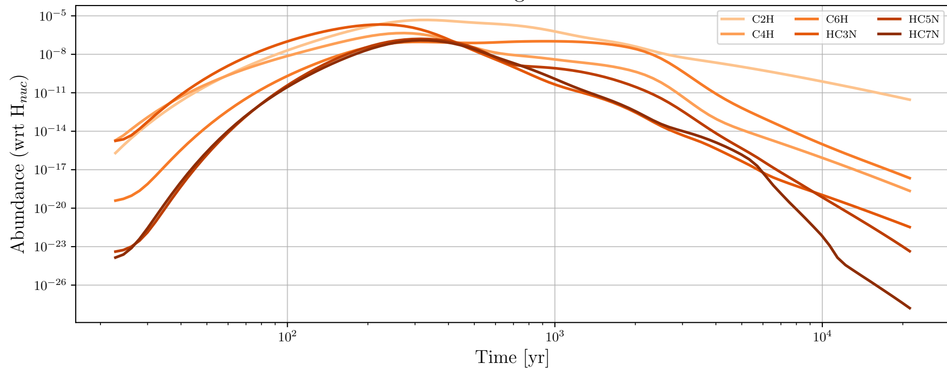
Particle 1 - Daughter Molecules
