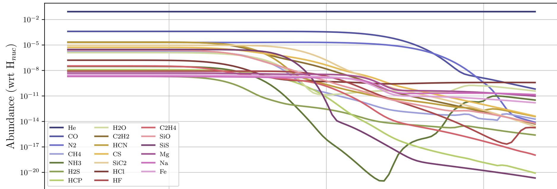
Particle 1 - Parent Molecules
