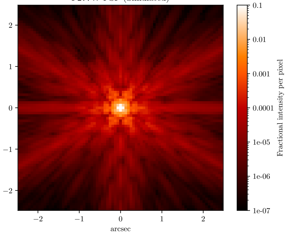
F277W PSF (Simulated)
