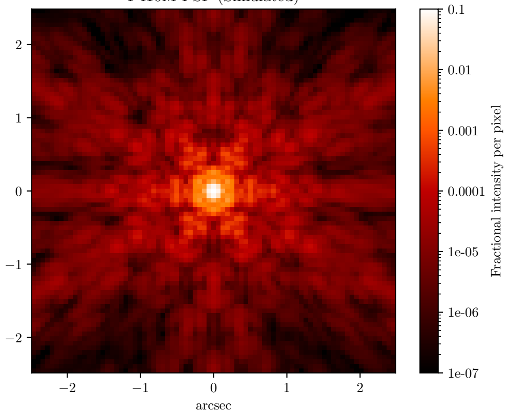
F410M PSF (Simulated)
