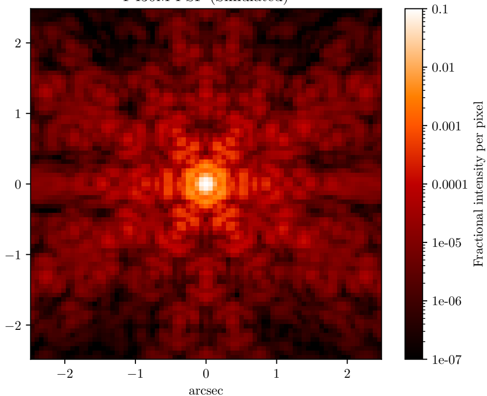
F430M PSF (Simulated)
