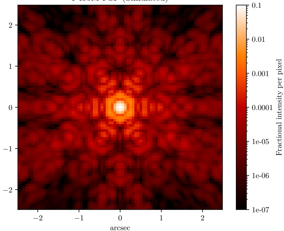
F480M PSF (Simulated)
