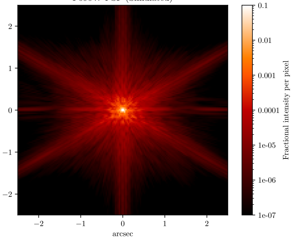
F090W PSF (Simulated)
