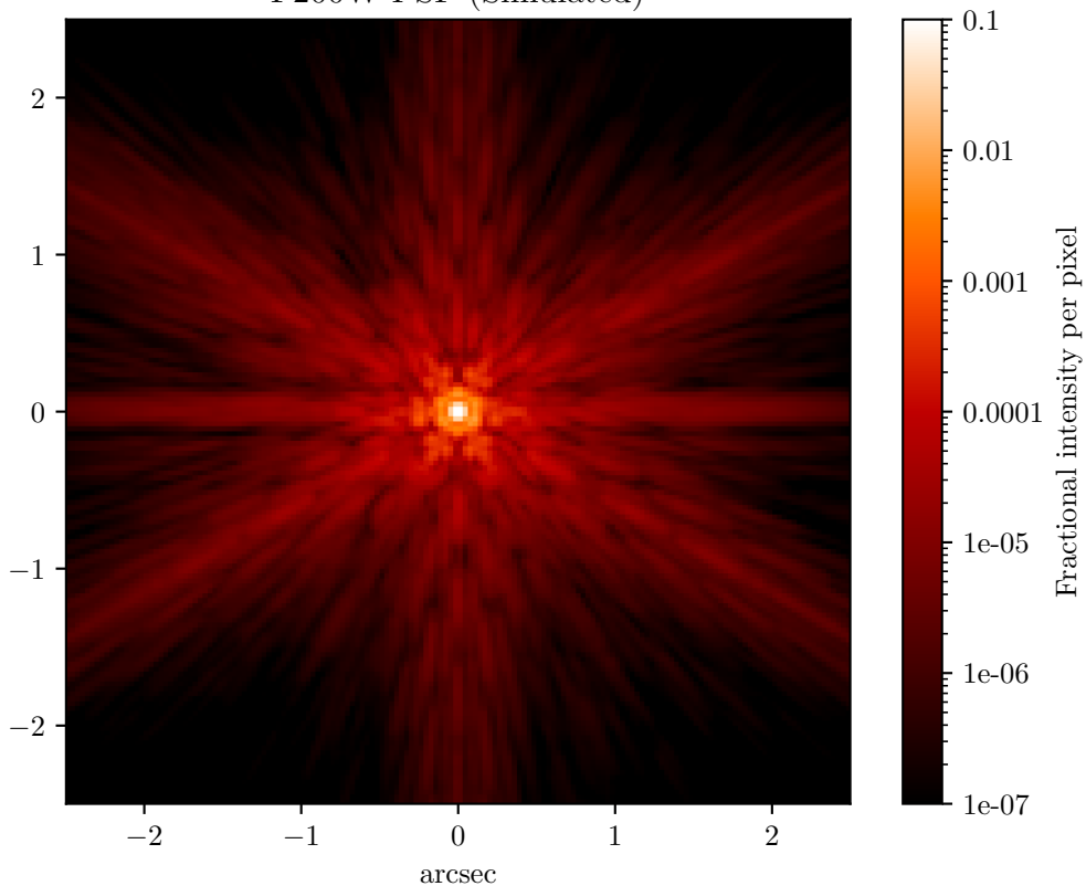
F200W PSF (Simulated)
