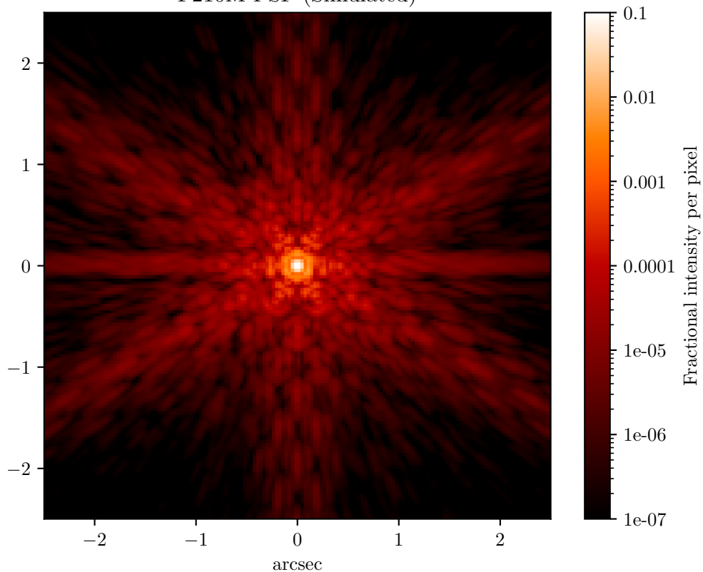
F210M PSF (Simulated)
