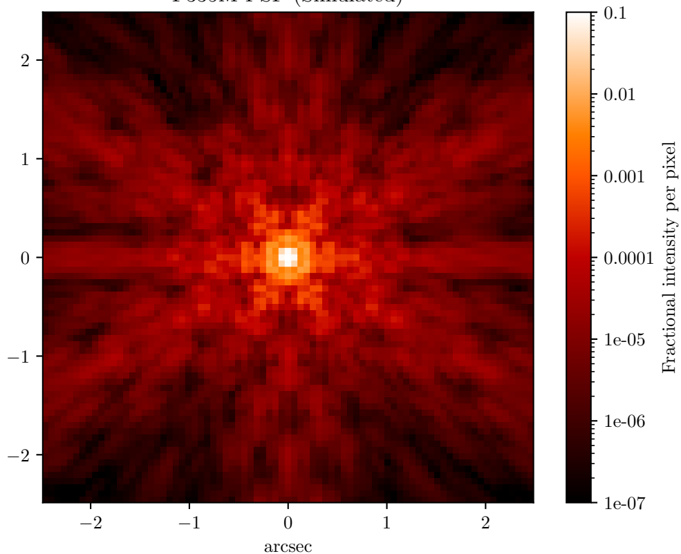
F335M PSF (Simulated)
