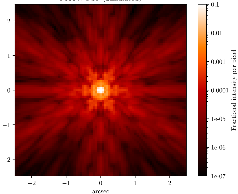
F356W PSF (Simulated)
